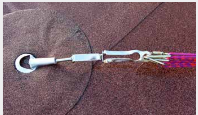
Deployed Anchor tested to CEN / TS 16415 for a 3rd user (rescuer) falling on an anchor that was deployed
